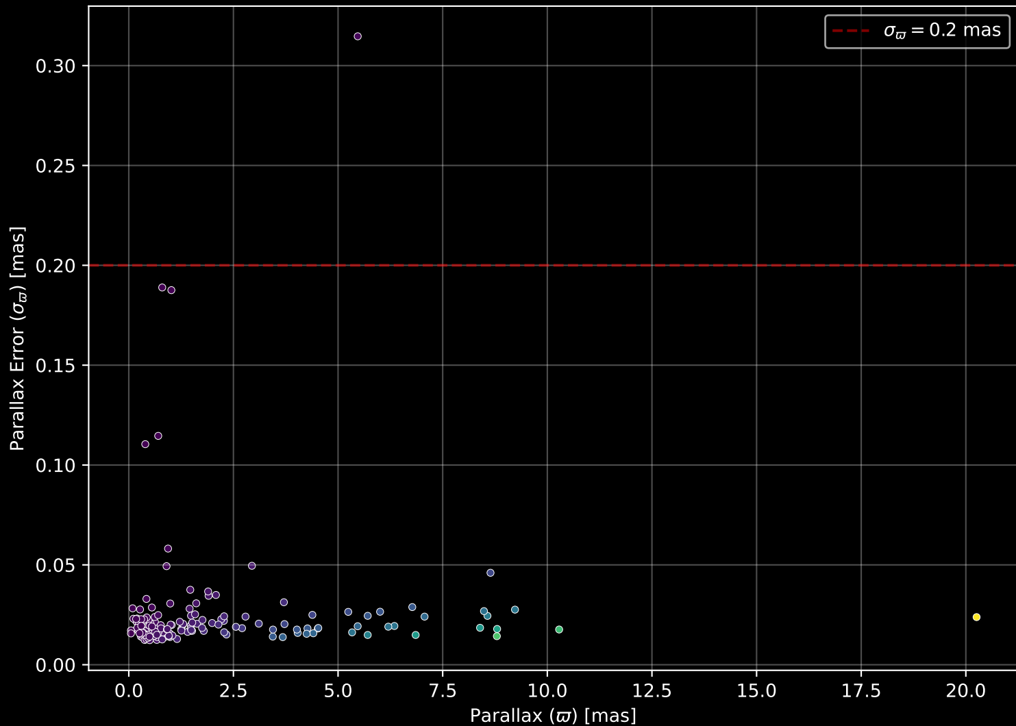
APOGEE DR17 Field: [187+24_MGA] Parallax Quality (n= 176)
