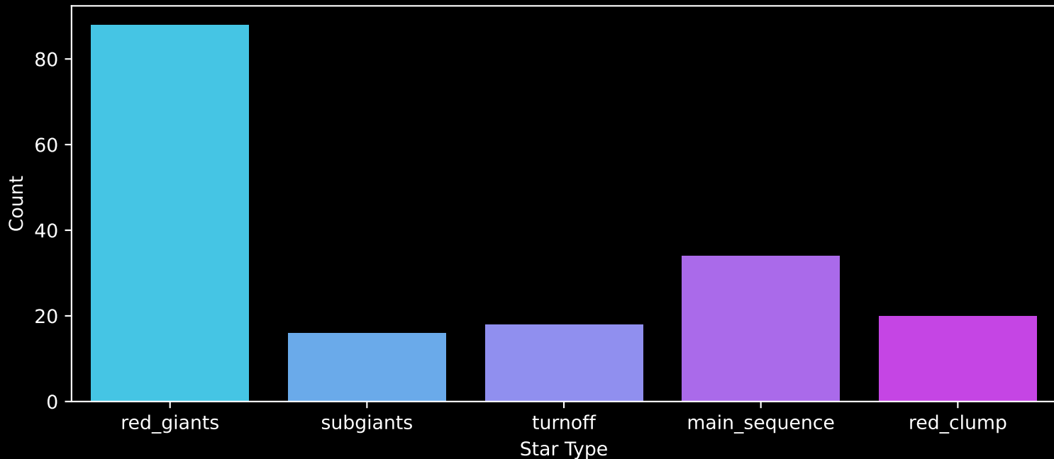
APOGEE DR17 Field: [187+24_MGA] Count plot of Star Type
