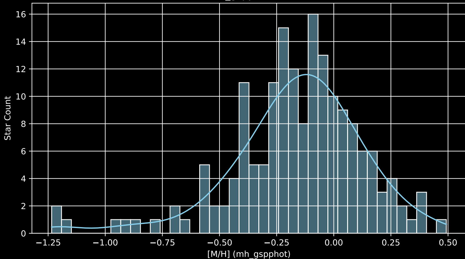
APOGEE DR17 Field: [187+24_MGA [M/H] (mh_gspphot) (n= 172)
