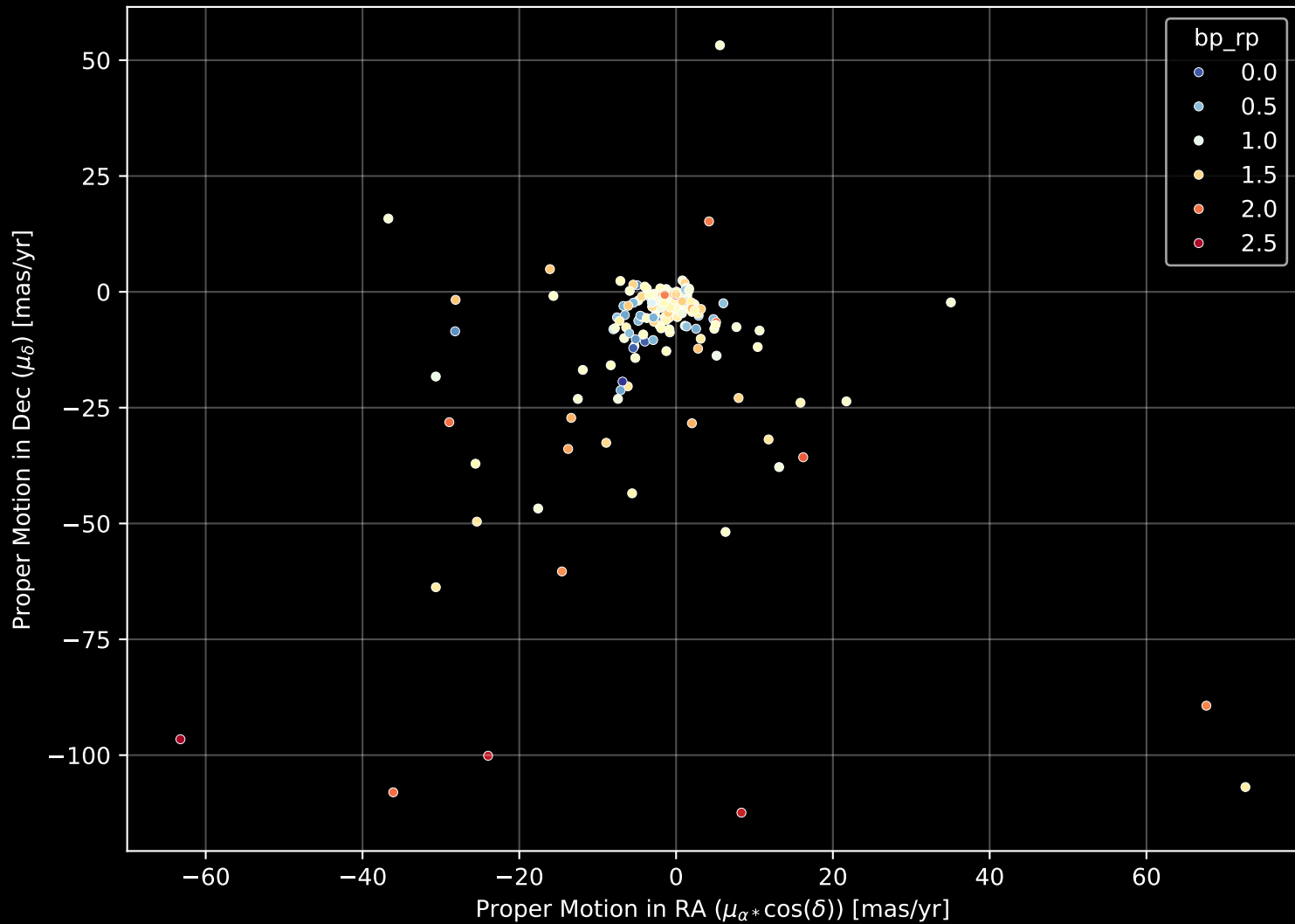
APOGEE DR17 Field: [187+24_MGA] Proper Motion Diagram (n= 176)
