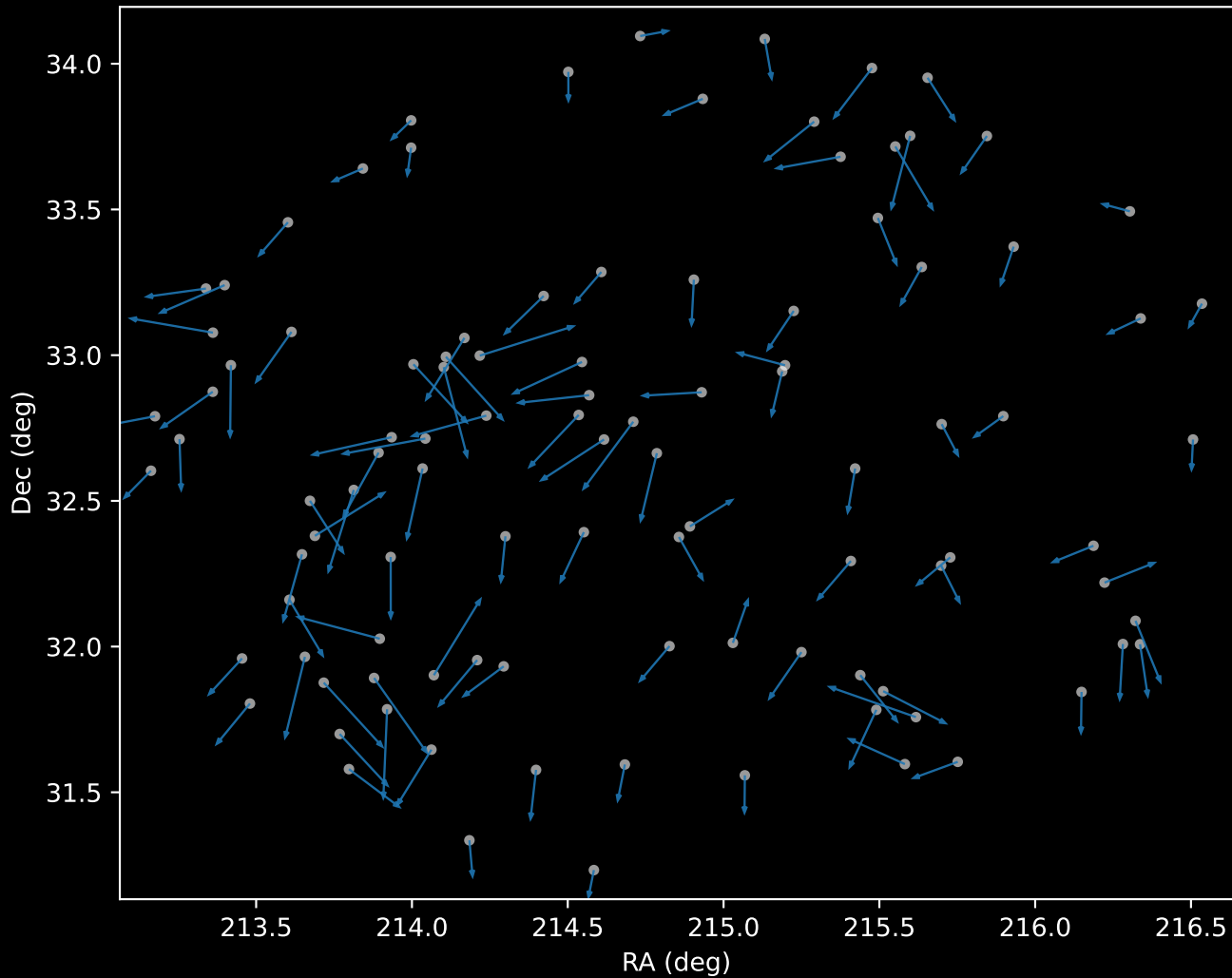
APOGEE DR17 Cluster 0 Proper Motion Vectors (n=103)
