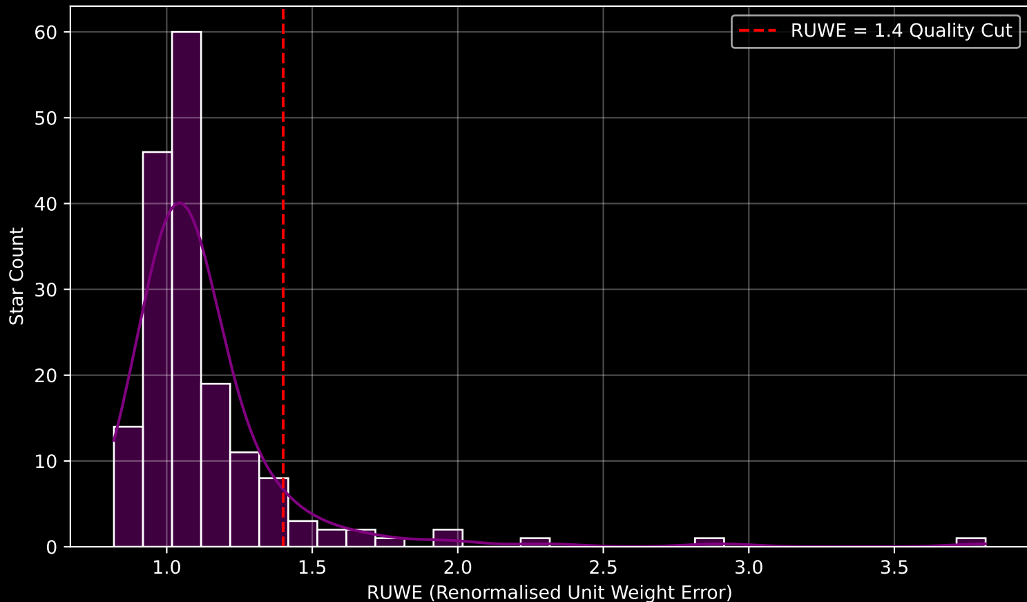
GAPOGEE DR17 Field [187+24_MGA] RUWE Distribution (n= 171)
