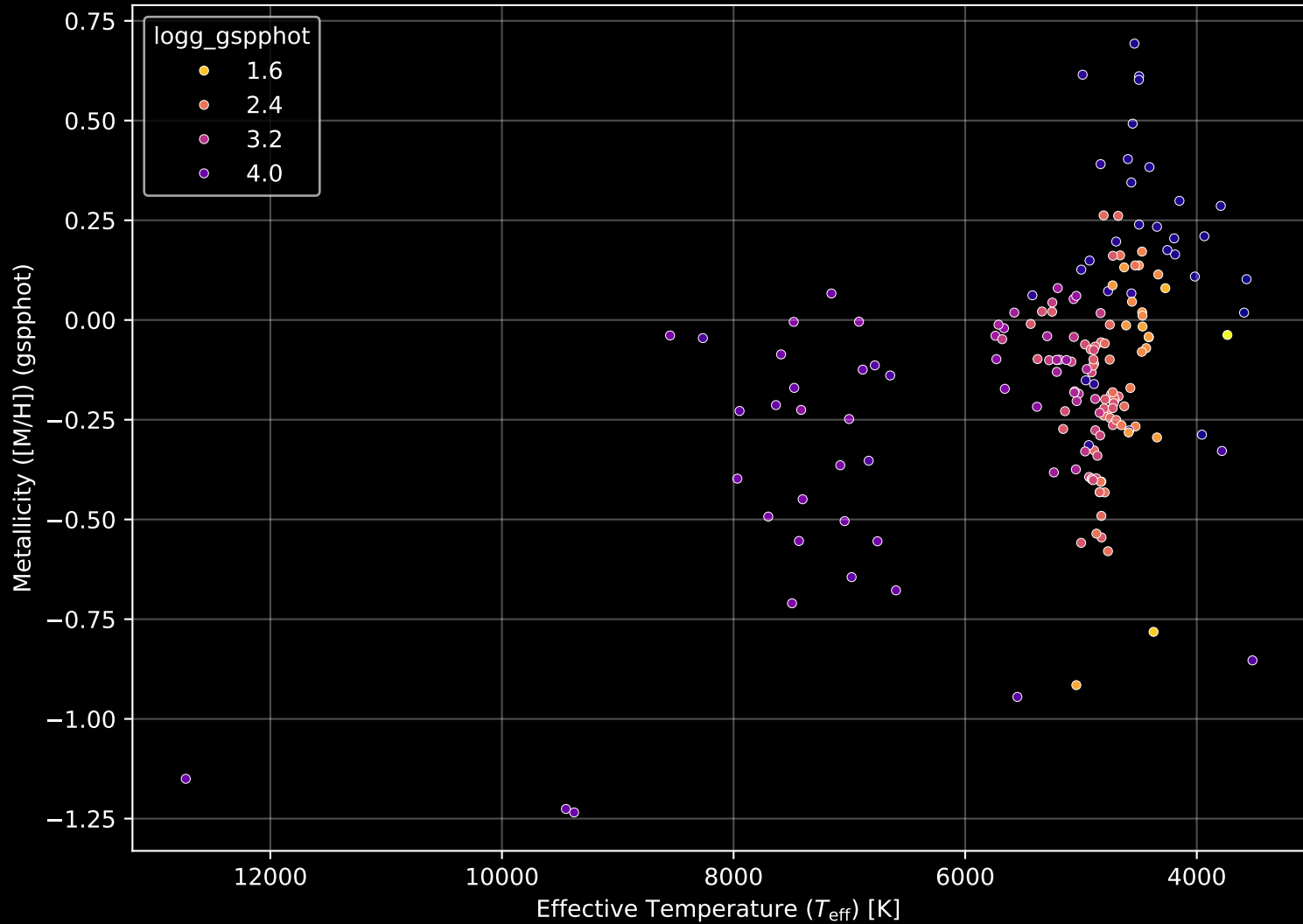
APOGEE DR17 Field: [187+24_MGA] Stellar Population Parameters (n= 176)
