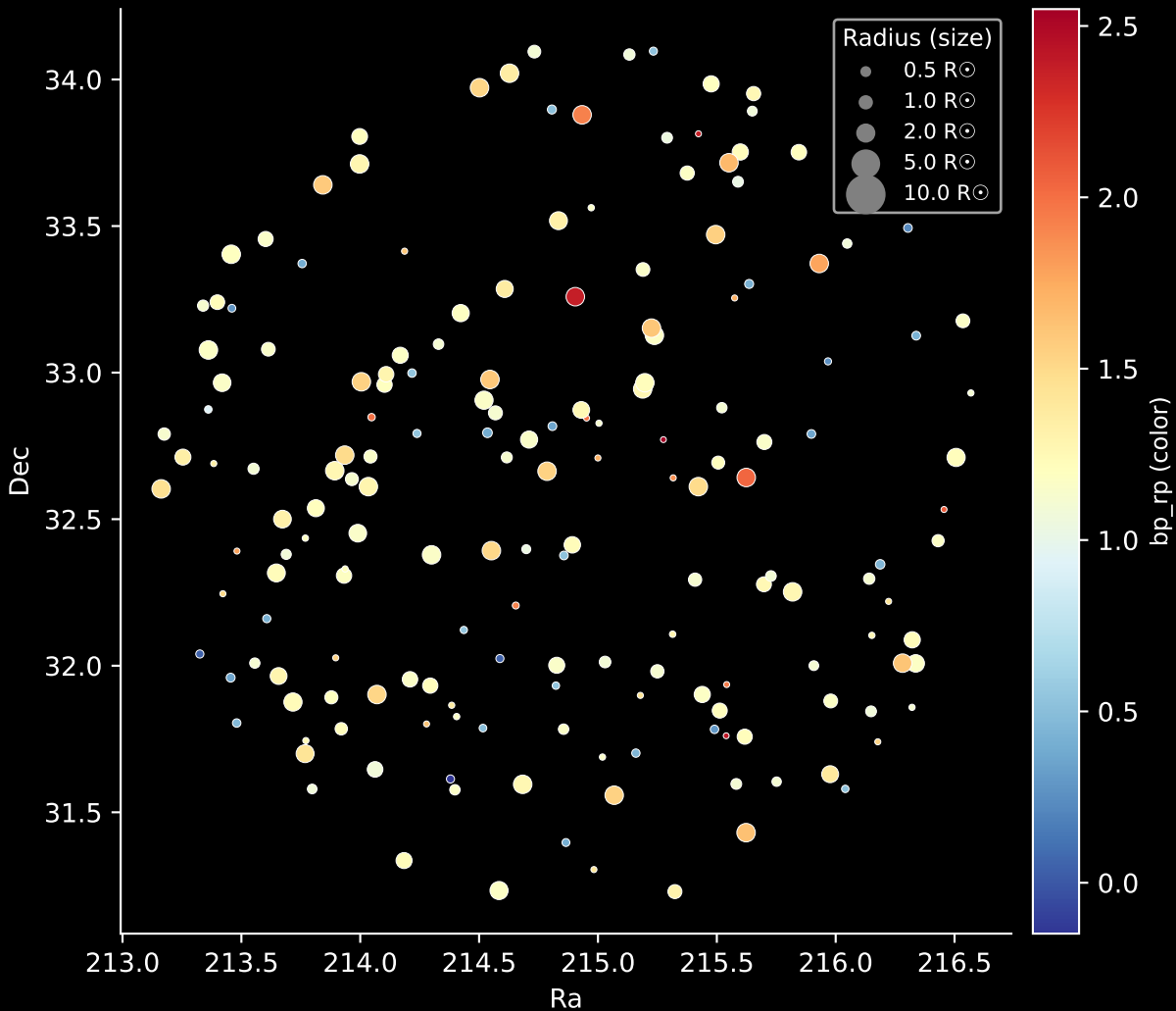
APOGEE DR17 Field: [187+24_MGA] Stars: 176
